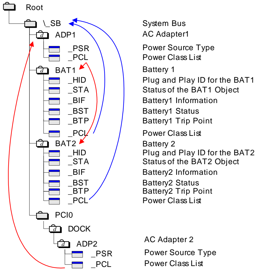
Figure 10-4 Power Source Name Space Example that Includes a Docking Station
