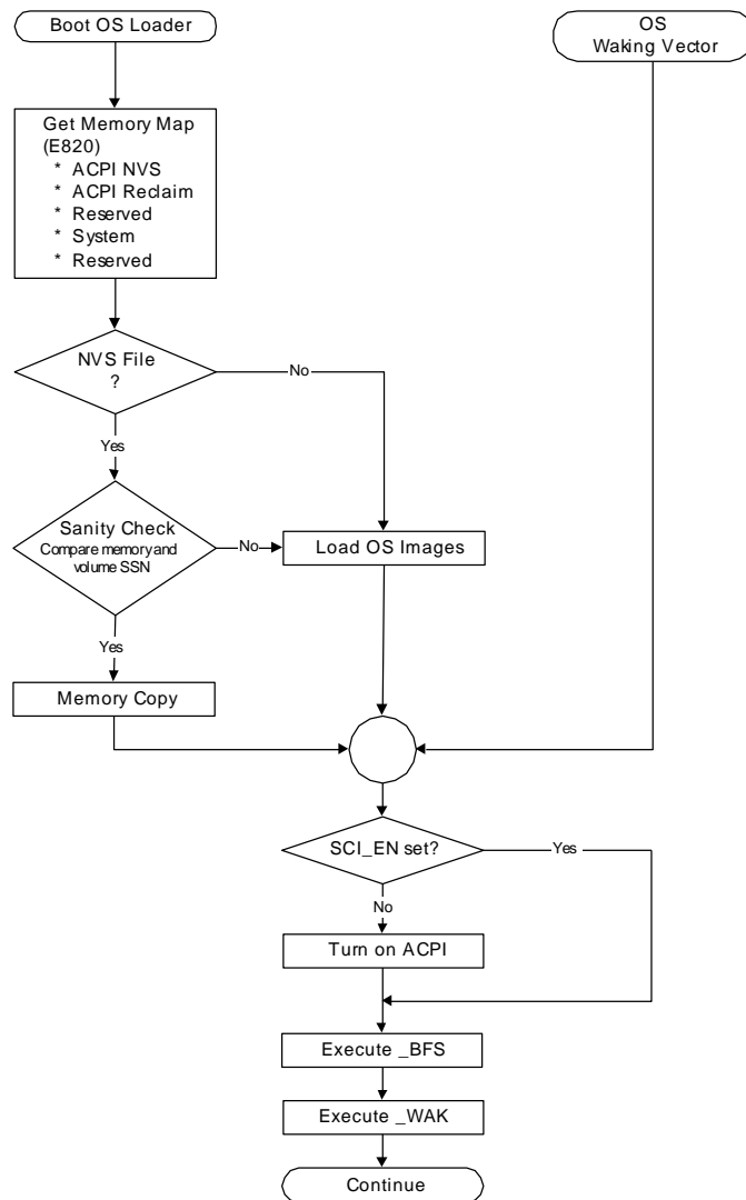
Figure 15-5 OS Initialization
