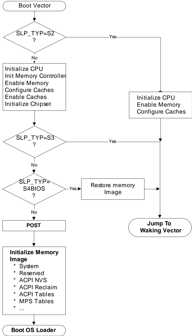
Figure 15-2 BIOS Initialization
