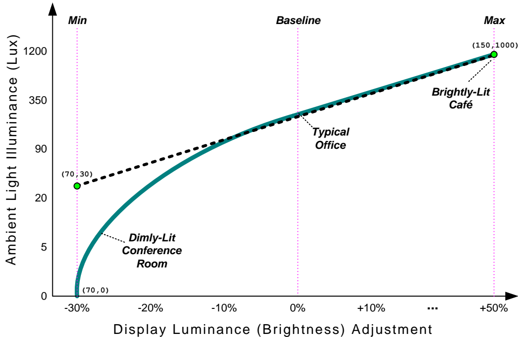
Figure 9-2: A two-point ALS Response Curve
