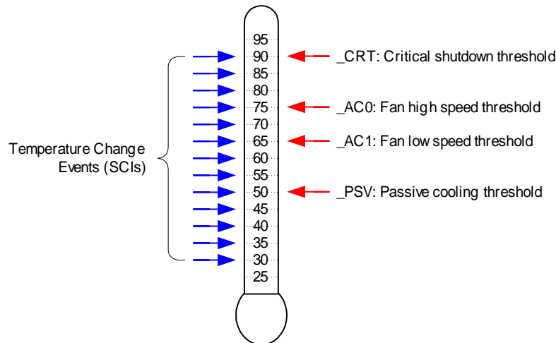
Figure 11-2 Thermal Events
