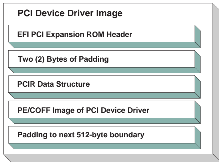
Figure 45. Recommended PCI Driver Image Layout
