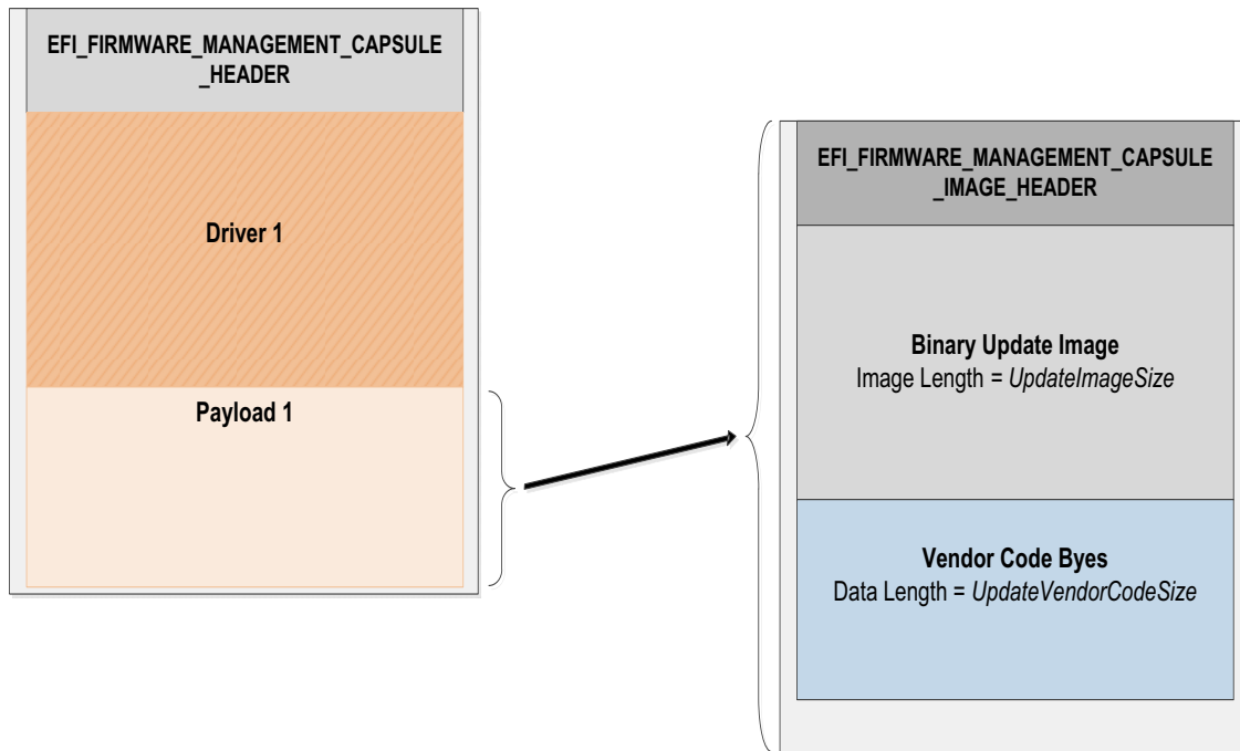
Figure 118. Firmware Management and Firmware Image Management headers
