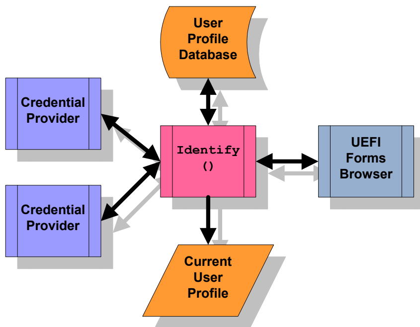
Figure 113. User Identity
