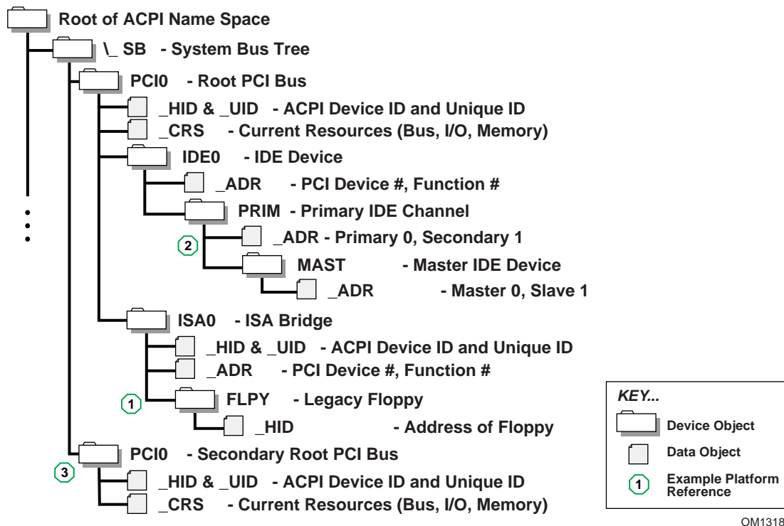
Figure 120. Partial ACPI Name Space for Example System
