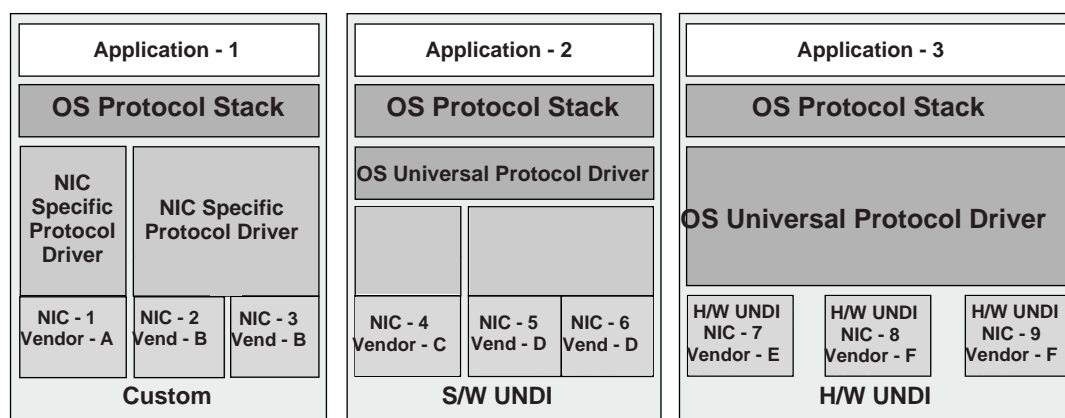
Figure 122. Network Stacks with Three Classes of Drivers
