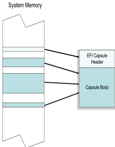
Figure 116. Optional Scatter-Gather Construction of Capsule Submitted to UpdateCapsule()
