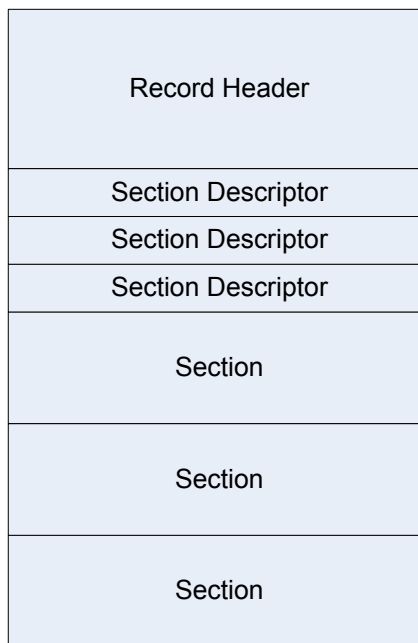
Figure 130. Error Record Format
