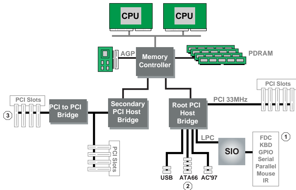
Figure 119. Example Computer System
