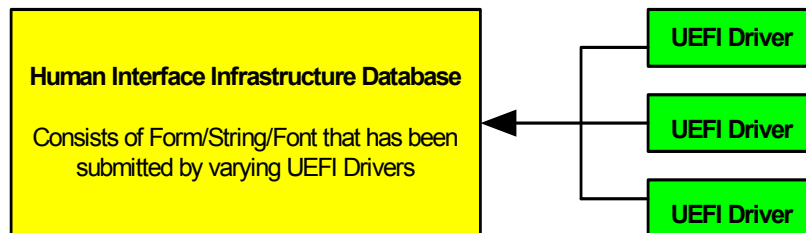
Figure 89. HII Database
