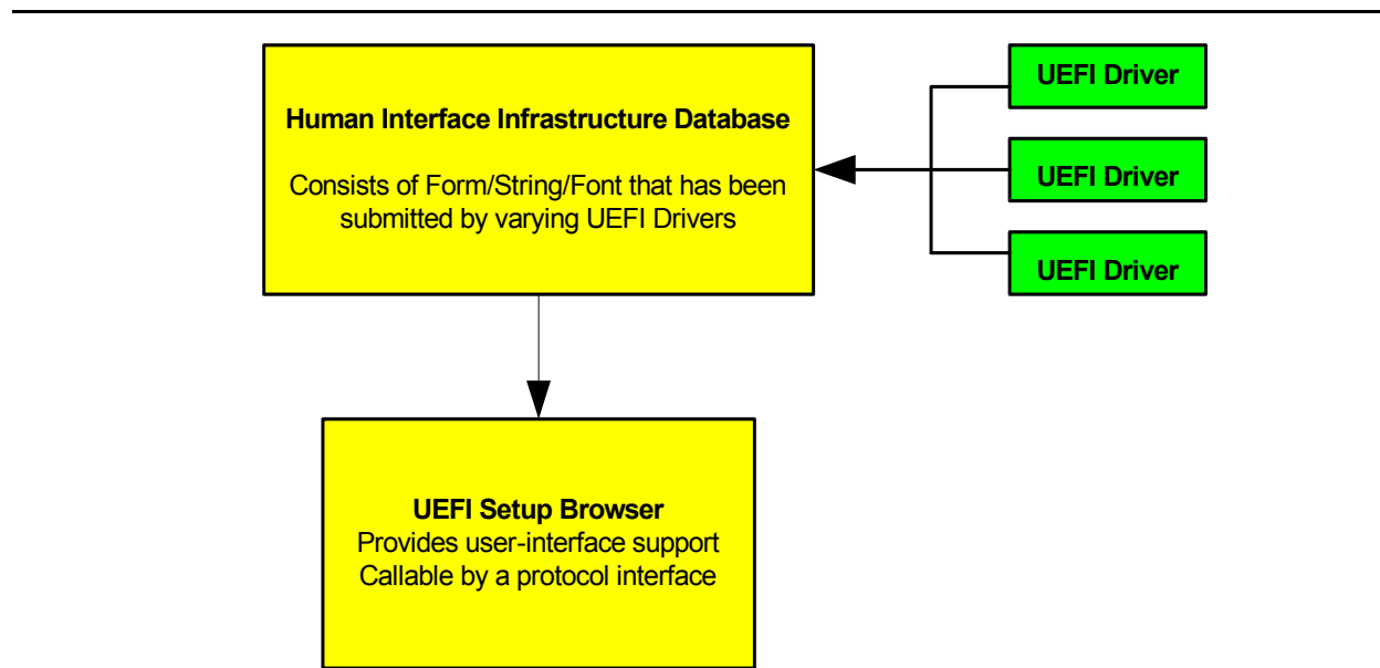
Figure 90. Setup Browser
