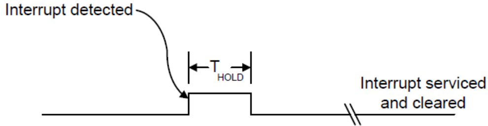
Fig. 12.3: Interrupt Model
