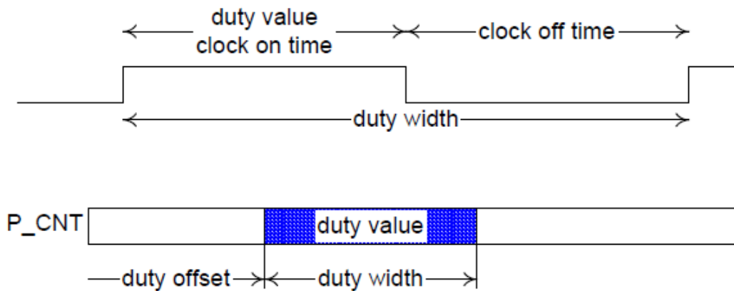
Fig. 8.2: Throttling Example
