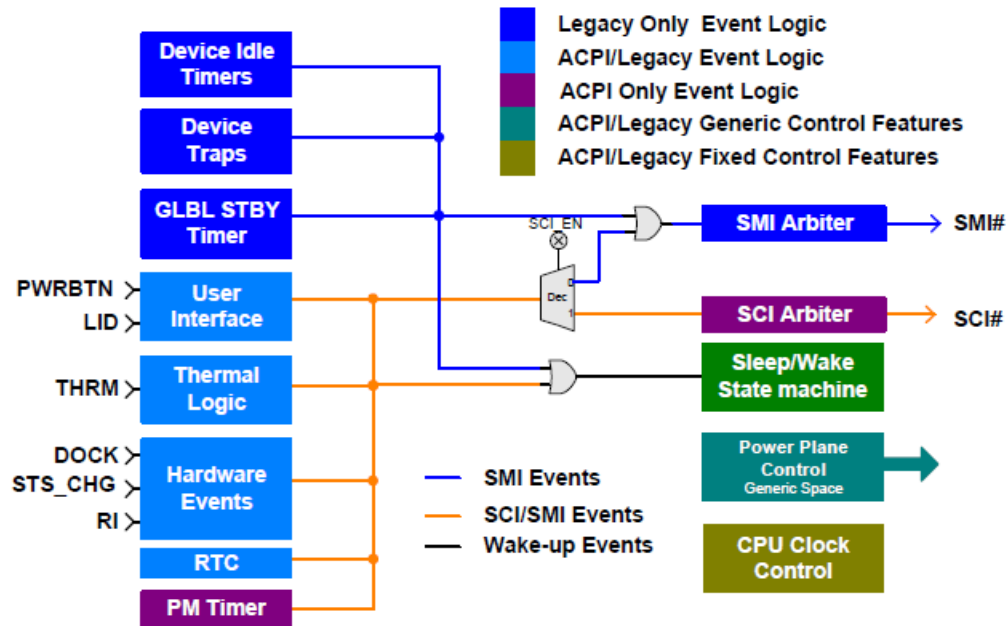
Fig. 4.3: Example Event Structure for a Legacy/ACPI Compatible Event Model
