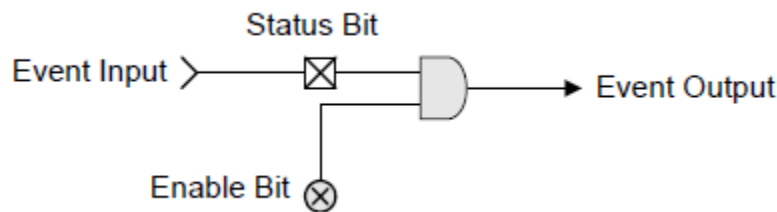
Fig. 4.4: Block Diagram of a Status/Enable Cell
