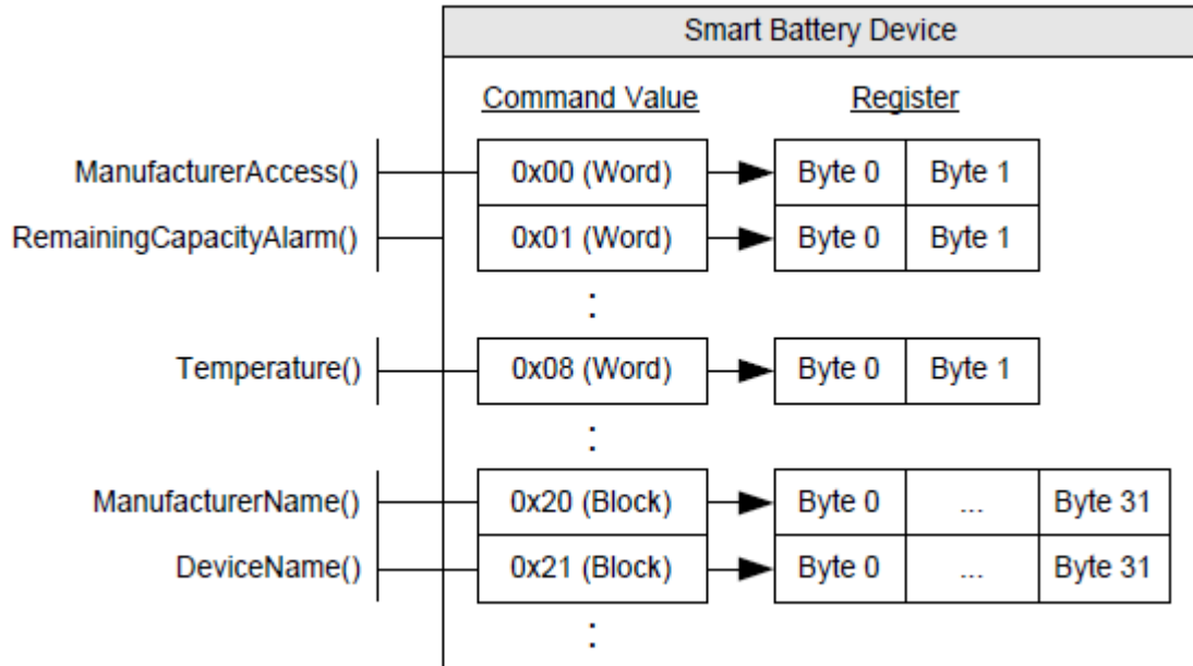
Fig. 13.3: Smart Battery Device Virtual Registers
