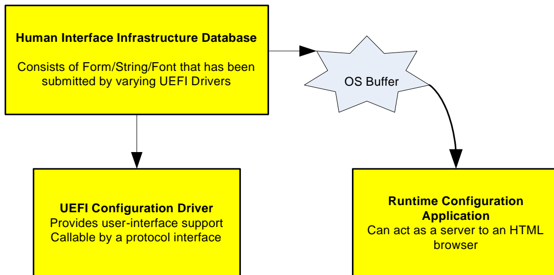
Figure 119. OS Runtime Utilization
