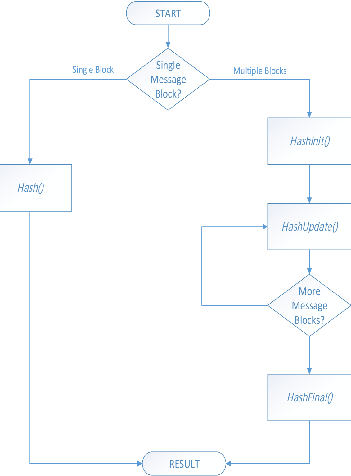
Figure 147. Hash workflow
