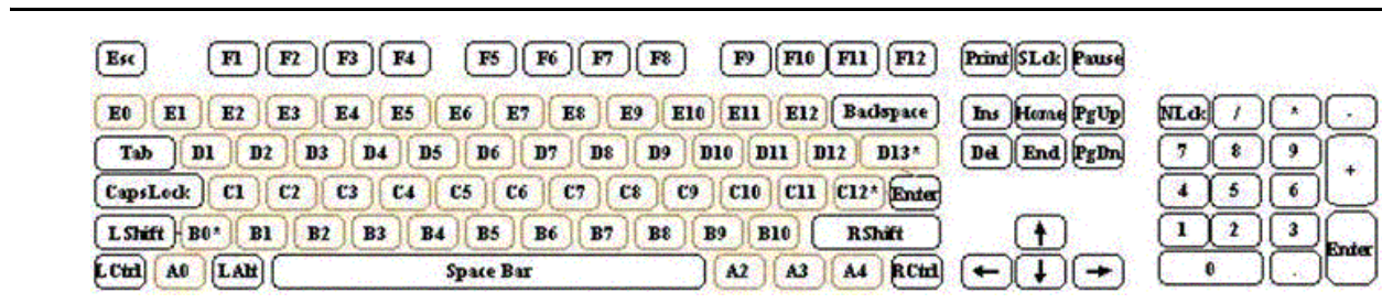
Figure 145. Keyboard Layout
