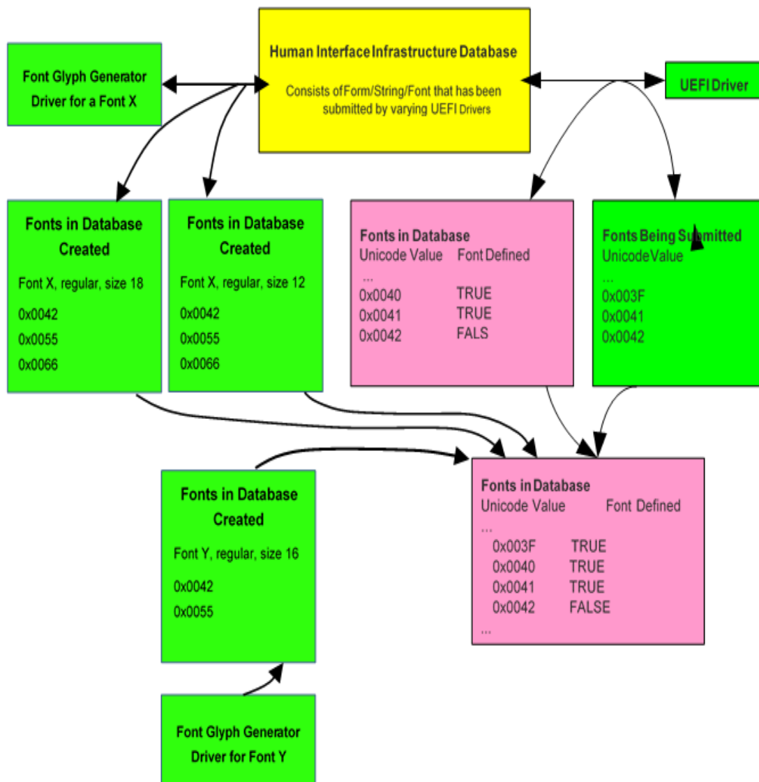
Figure 110. Fonts
