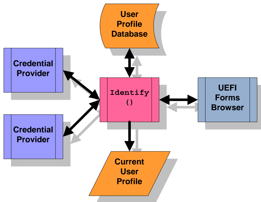
Figure 146. User Identity
