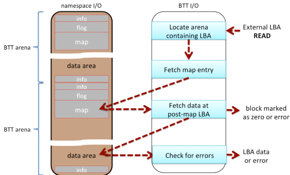
Figure 23. BTT Read Path Overview
