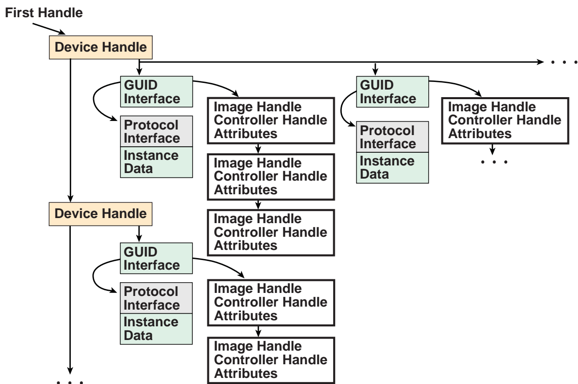
Figure 26. Handle Database
