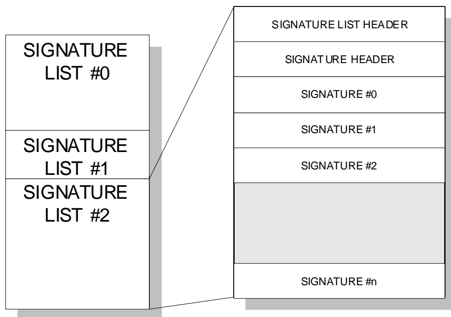
Figure 91. Signature lists
