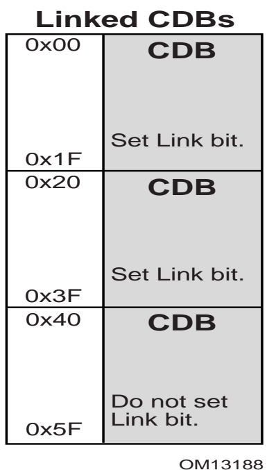
Figure 157. Linked CDBs
