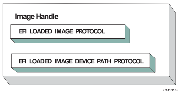
Figure 44. Image Handle
