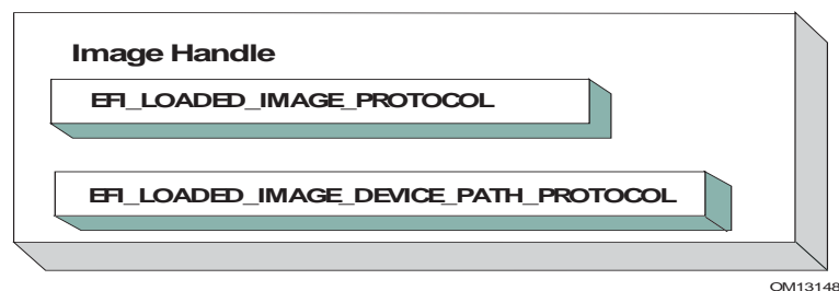
Figure 8. Image Handle
