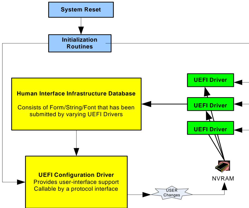
Figure 118. Storing Configuration Settings
