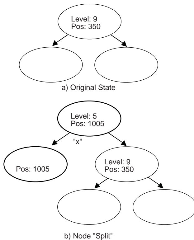
Figure 68. Node Split
