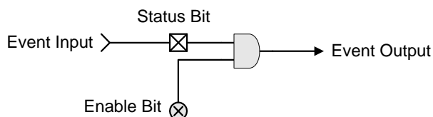
Figure 4-12 Block Diagram of a Status/Enable Cell
