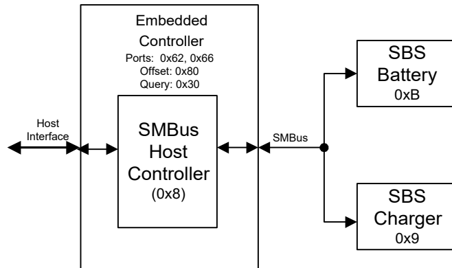
Figure 10-61 Single Smart Battery Subsystem
