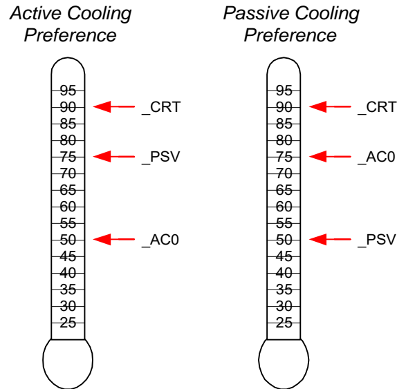
Figure 11-70 Cooling Preferences
