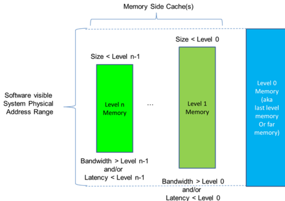
Figure 5-30 Memory Side Cache Example
