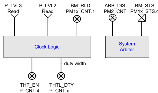
Figure 8-45 ACPI Clock Logic (One per Processor)
