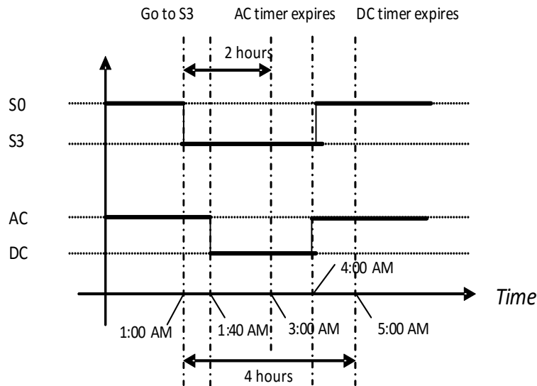
Figure 9-58 System transitions with WakeAlarm -- Policy
