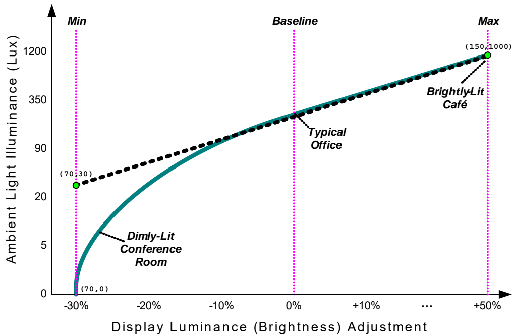
Figure 9-53 A two-point ALS Response Curve
