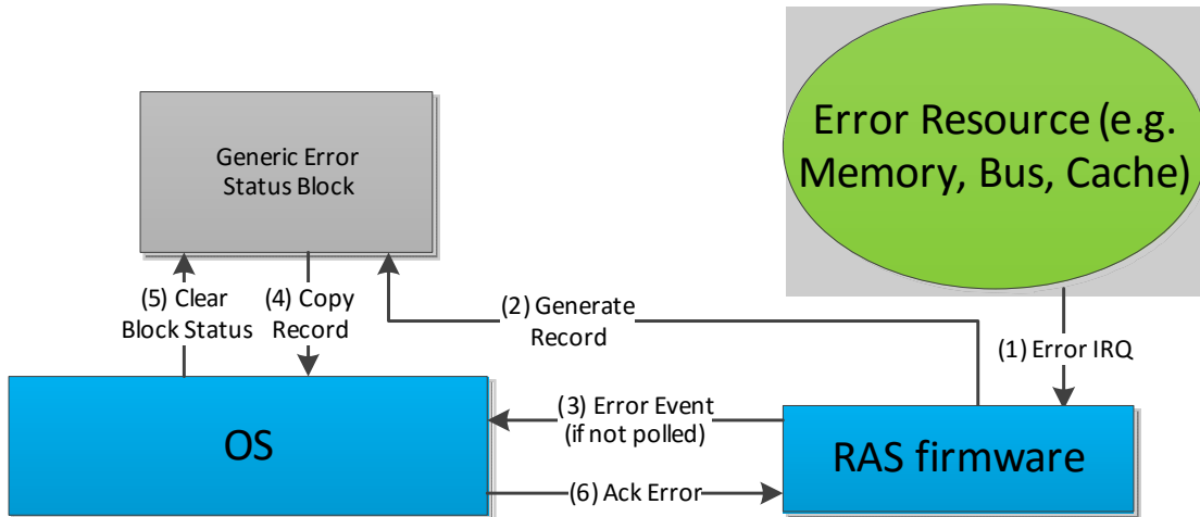
Figure 18-84 APEI error flow example with external RAS controller
