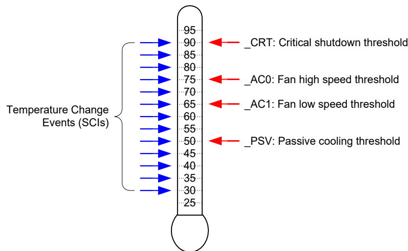
Figure 11-67 Thermal Events
