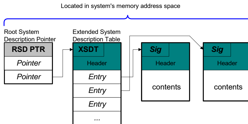
Figure 5-21 Root System Description Pointer and Table
