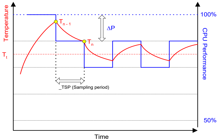
Figure 11-68 Temperature and CPU Performance Versus Time
