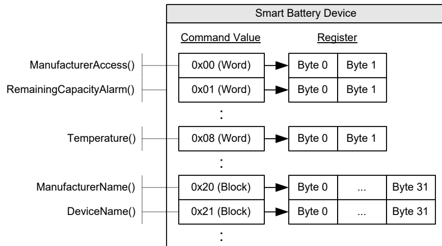
Figure 13-76 Smart Battery Device Virtual Registers
