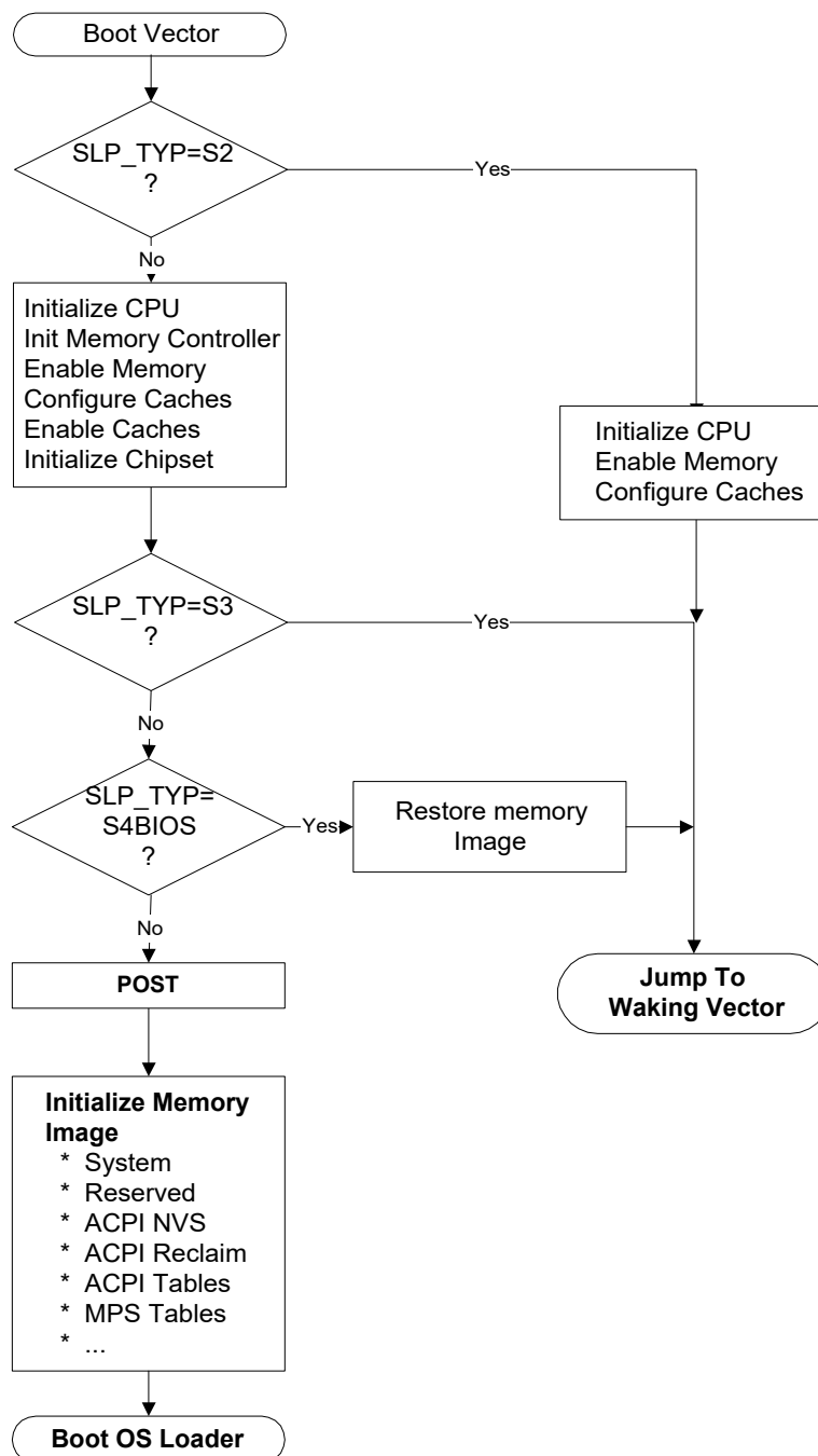
Figure 16-80 Platform Firmware Initialization
