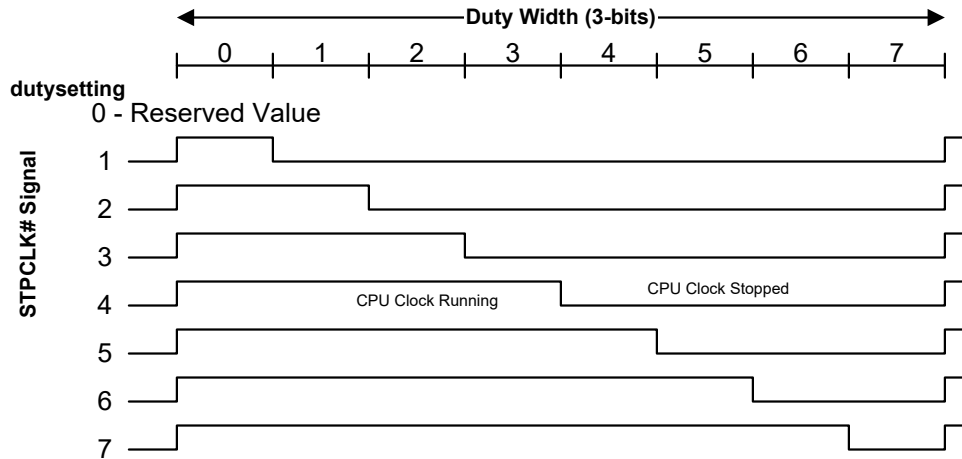
Figure 8-44 Example Control for the STPCLK#
