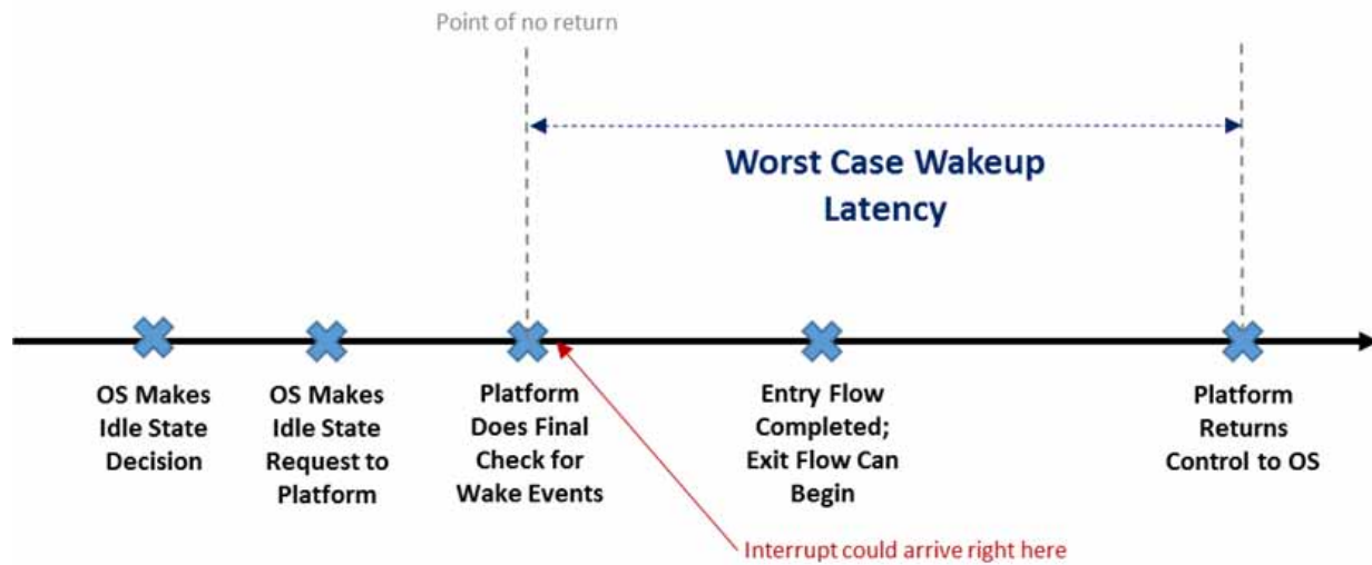
Figure 8-48 Worst case wake latency
