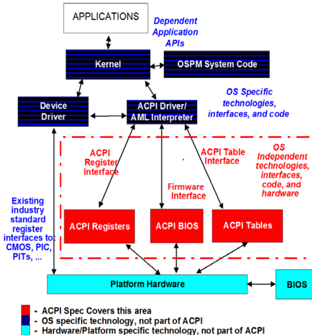
Figure 1-1 OSPM/ACPI Global System
