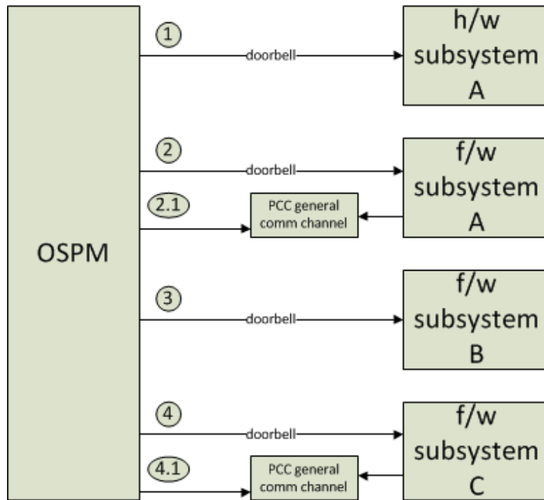
Figure 5-31 Example: Platform with 4 debug triggers
