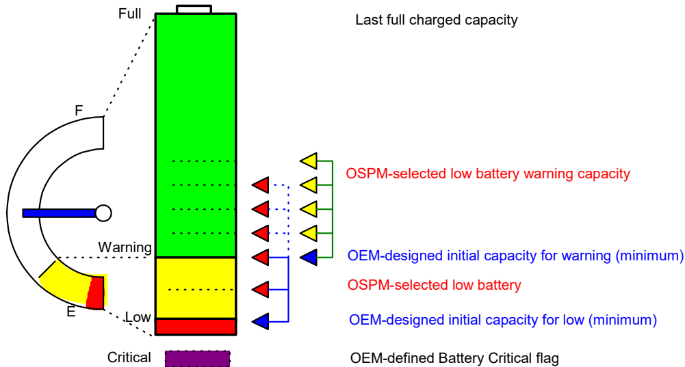
Figure 3-5 Low Battery and Warning
