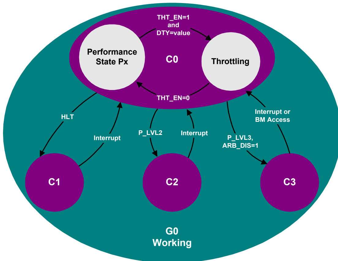
Figure 8-41 Processor Power States
