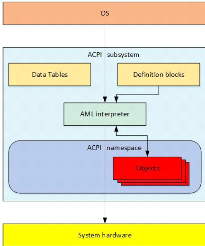
Figure 0-2. ACPI structure
