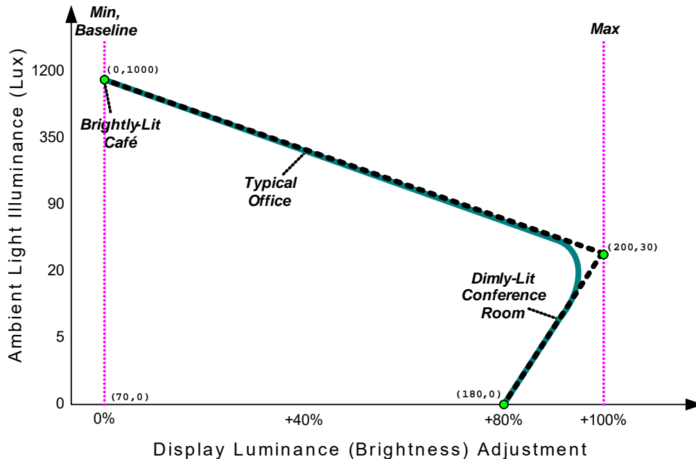
Figure 9-54 Example Response Curve for a Transflective Display
