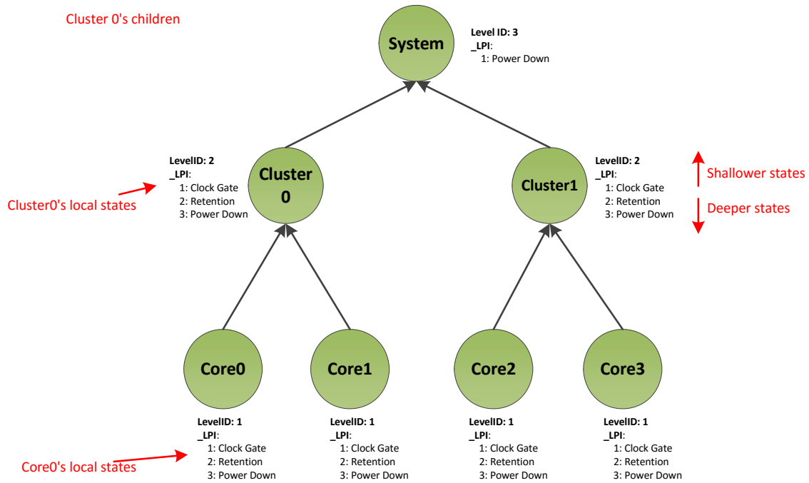
Figure 8-47 Power states for processor hierarchy
