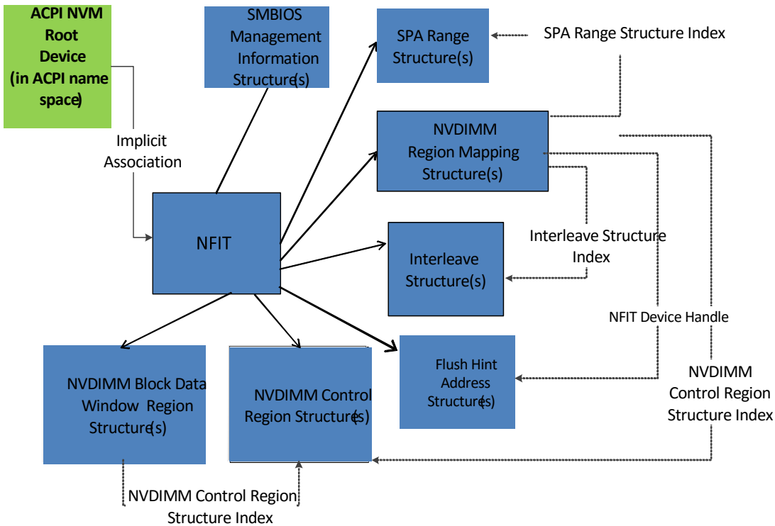
Figure 5-28 NVDIMM Firmware Interface Table (NFIT) Overview
