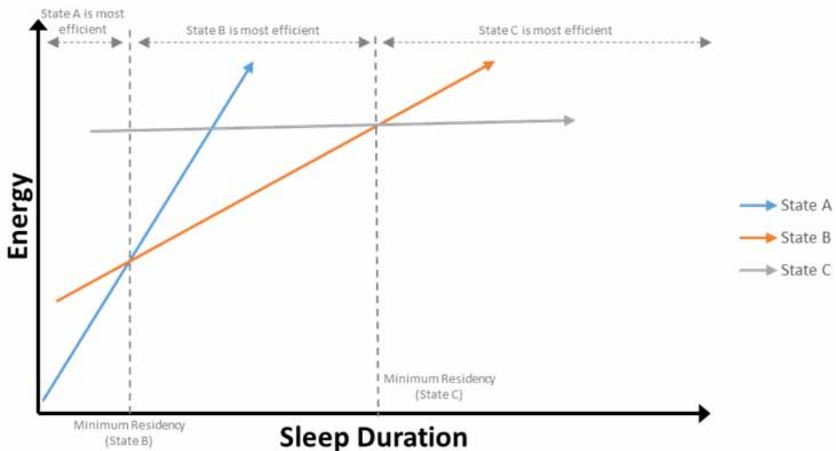
Figure 8-49 Energy of states A,B and C versus sleep duration
