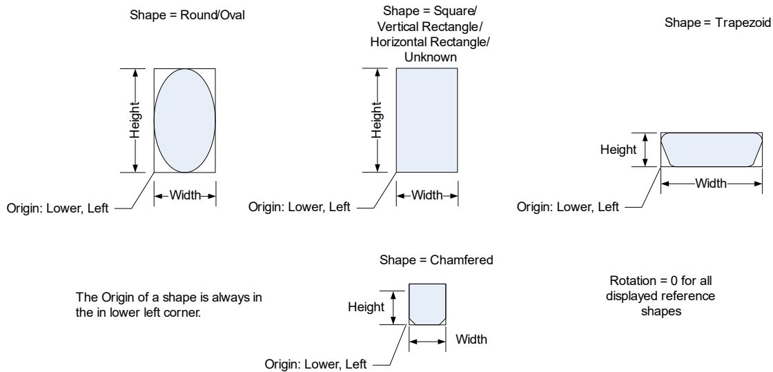
Figure 6-36 Default Shape Definitions
