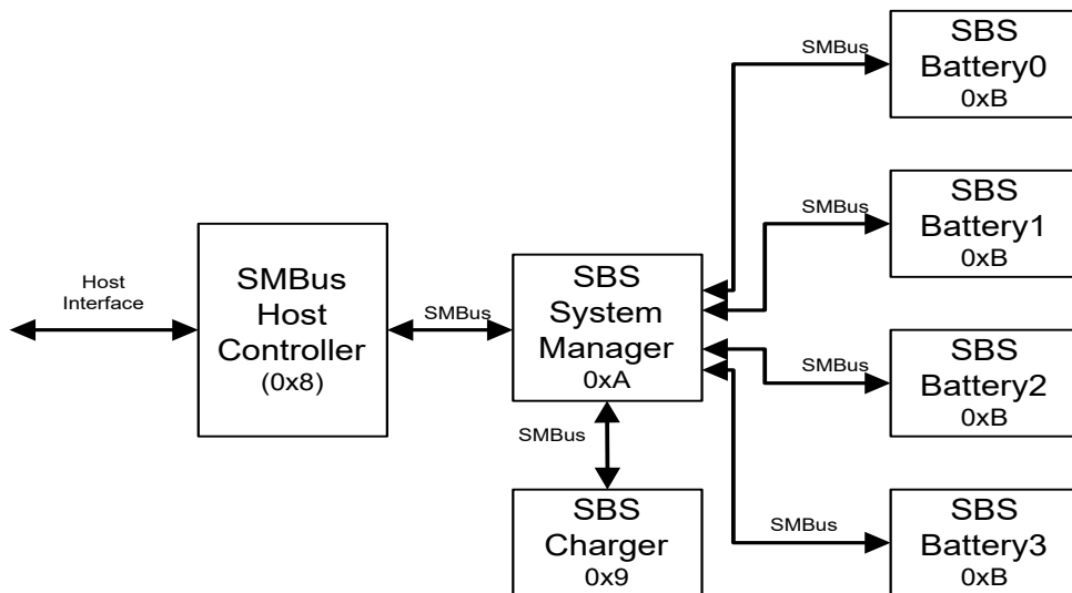
Figure 10-60 Typical Smart Battery Subsystem (SBS)
