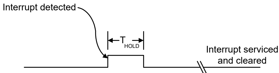
Figure 12-73 Interrupt Model
