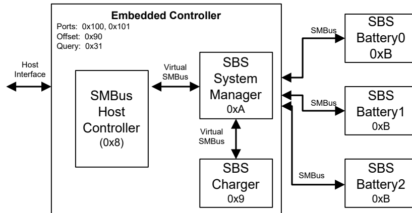
Figure 10-62 Smart Battery Subsystem
