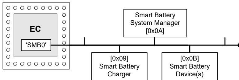
Figure 13-75 Smart Battery Subsystem Devices
