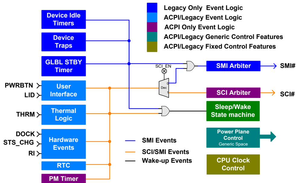
Figure 4-9 Example Event Structure for a Legacy/ACPI Compatible Event Model
