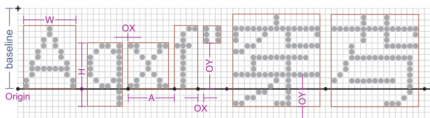
Figure 88. Aligning Glyphs
