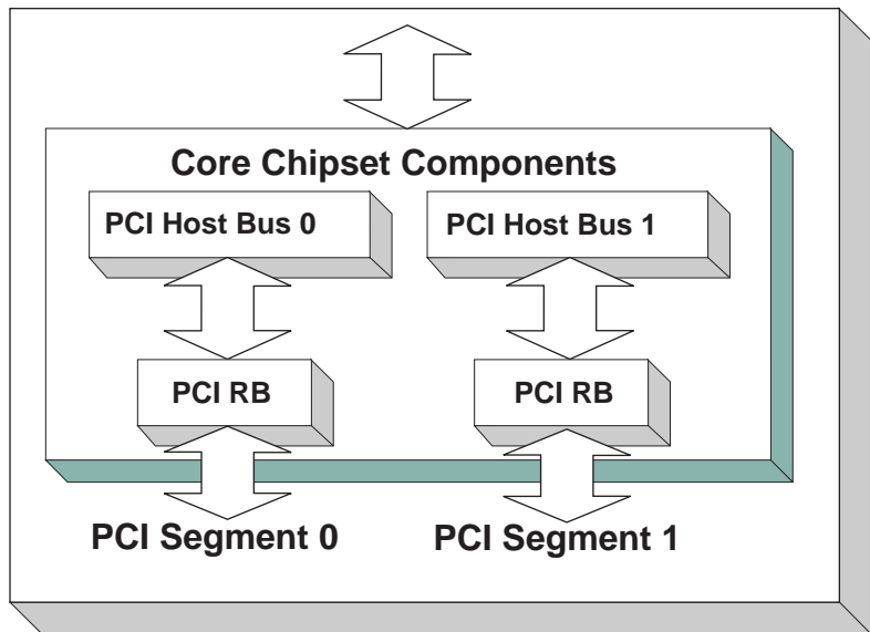
Figure 36. Server System with Two PCI Host Buses
