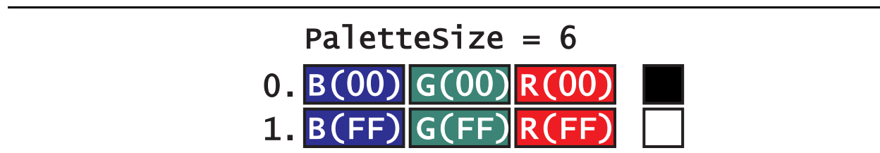
Figure 108. Palette Structure of a Black & White, One-Bit Image
