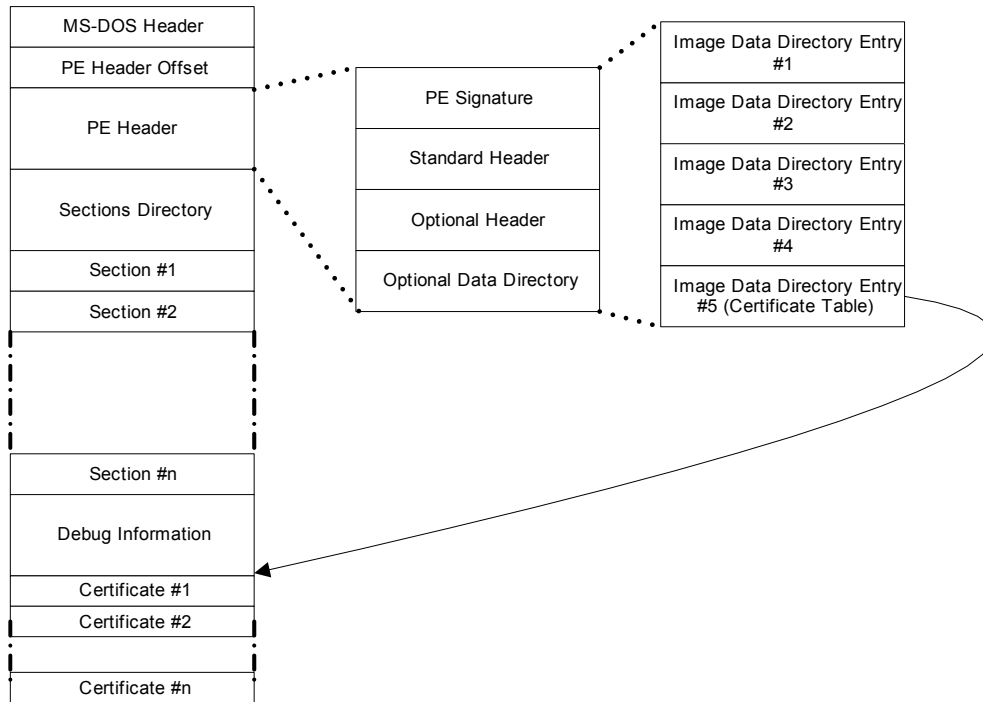
Figure 62. Embedded Digital Certificates
