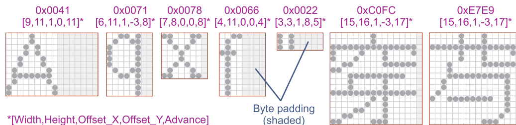
Figure 87. Proportional Font Parameters and Byte Padding
