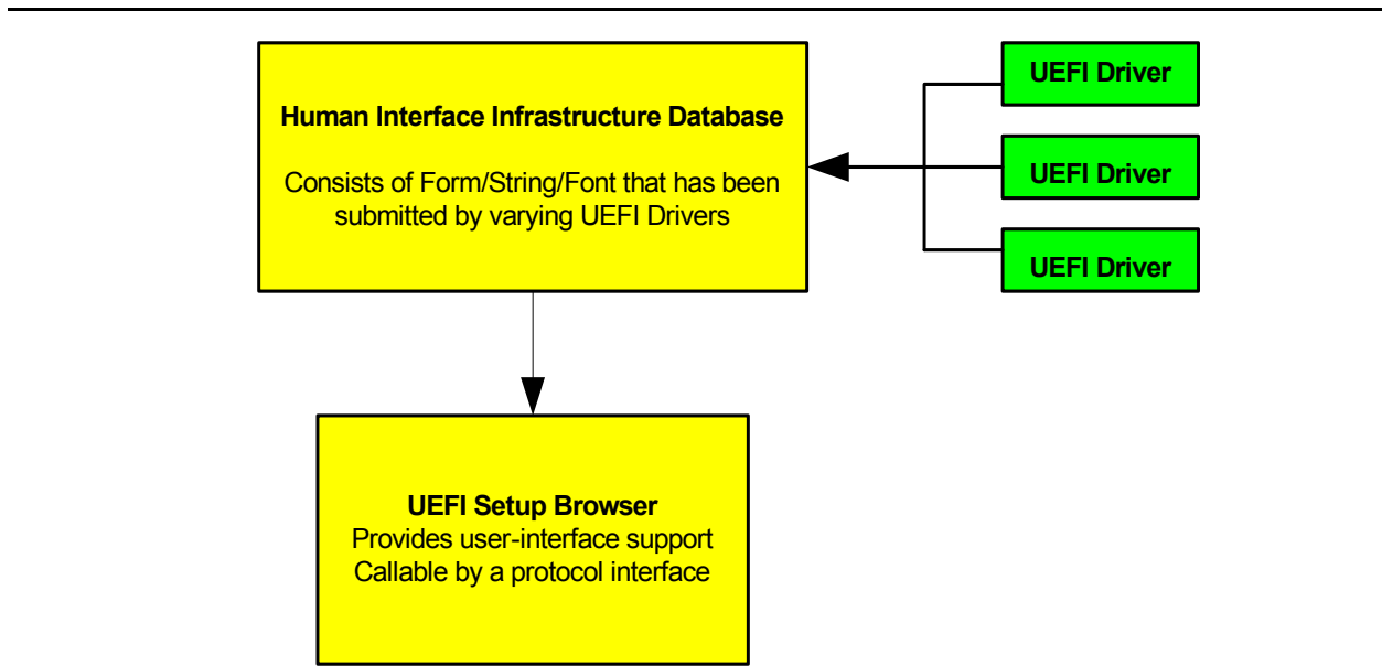
Figure 90. Setup Browser
