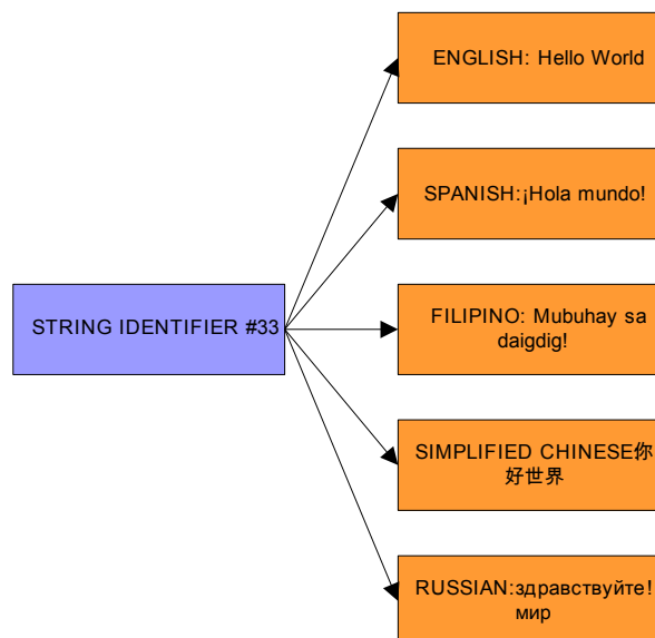
Figure 82. String Identifiers
