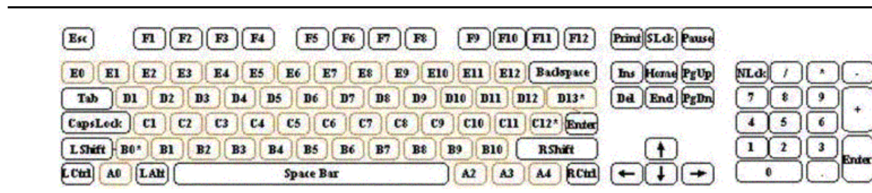
Figure 77. Keyboard Layout
